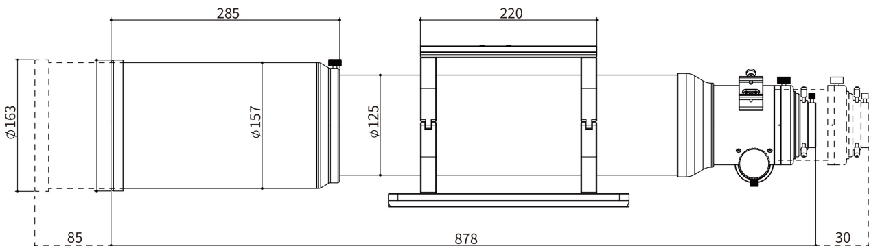
遮光罩可伸出长度 The extended length of the lens hood
