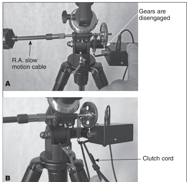
Figure 11 To move the right ascension axis with the slow-motion cable, disengage the motor drive by A ) pressing down on the motor housing using your hand, or B ) pulling down on the clutch cord.
