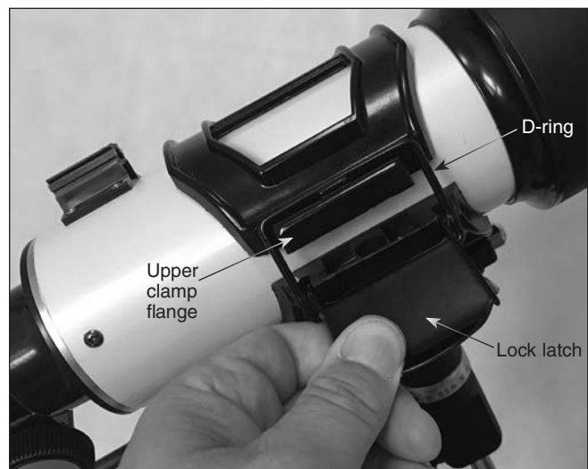
Figure 10. Lay the optical tube in the open clamp, then close the clamp and lock it in with the lock latch.
