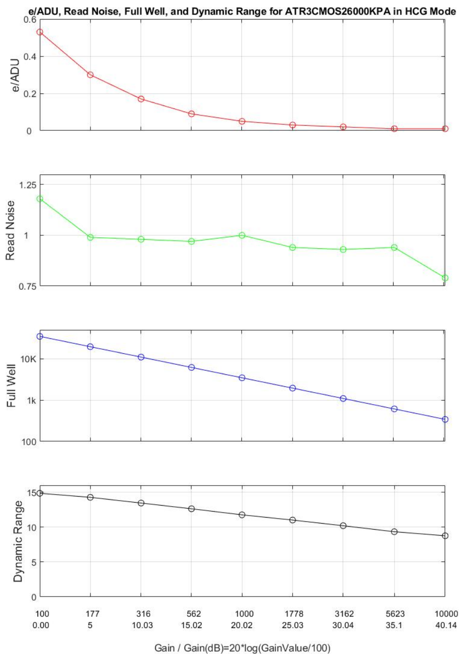
Figure 5.1 e-/ADU, Read Noise, Full Well and Dynamic Range for SkyEye26AM-plus
