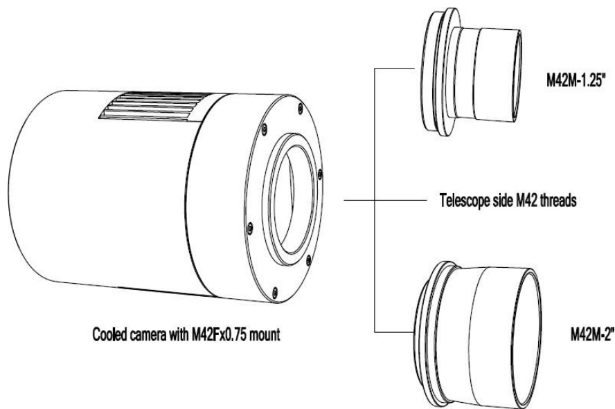
Figure 10 The Connection of the SkyEye Camera and Adapter
