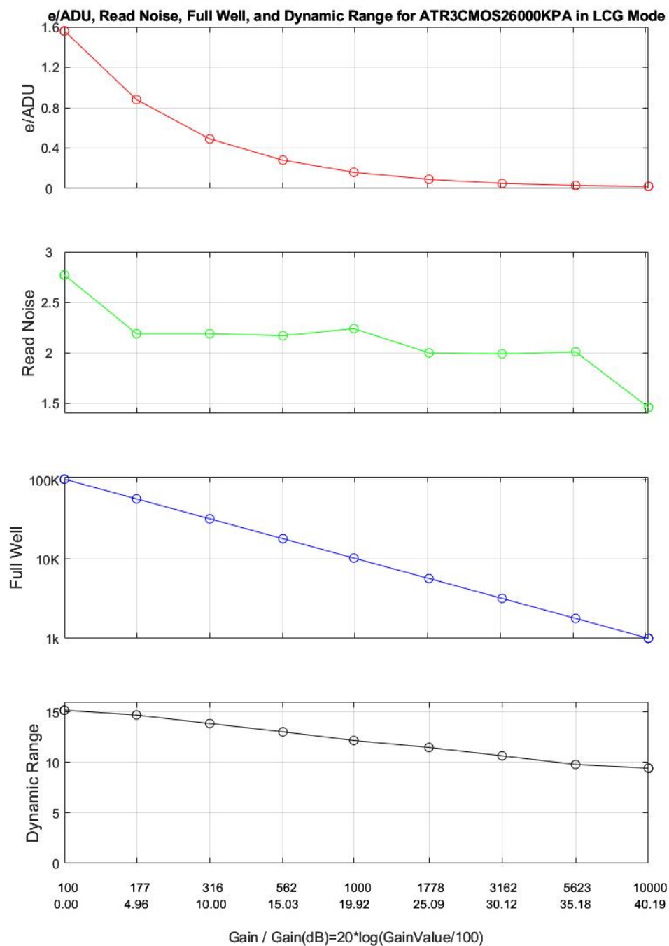
Figure 6.1 e-/ADU, Read Noise, Full Well and Dynamic Range for SkyEye26AM-plus
