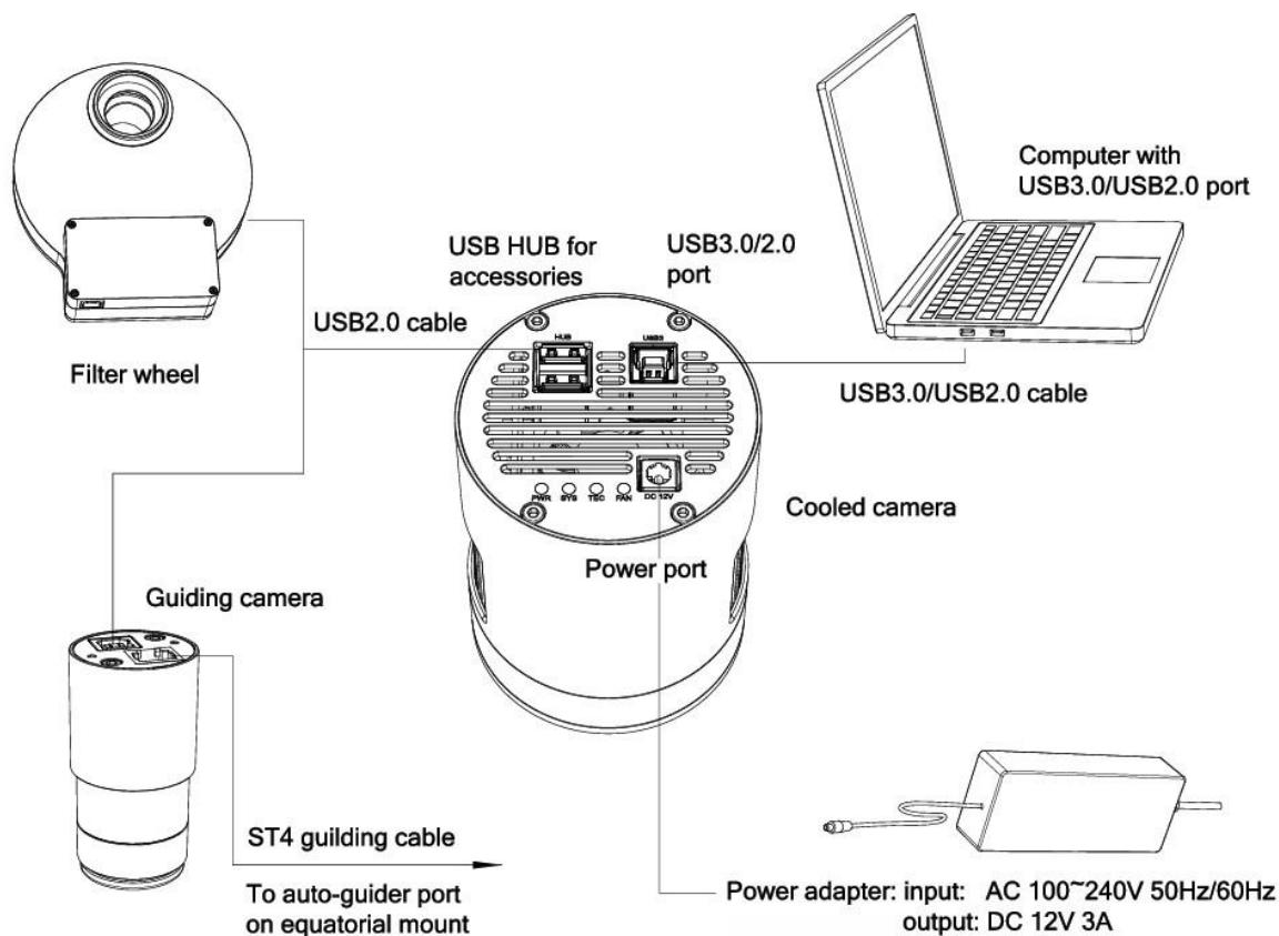
Figure 13 Camera Electric Connection
