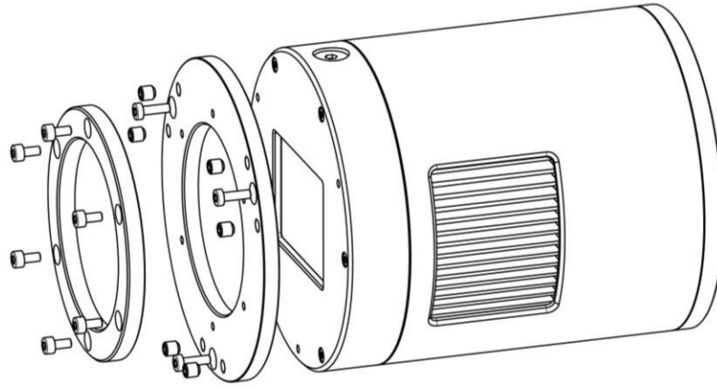
Figure 12 Tilt Adjustment
