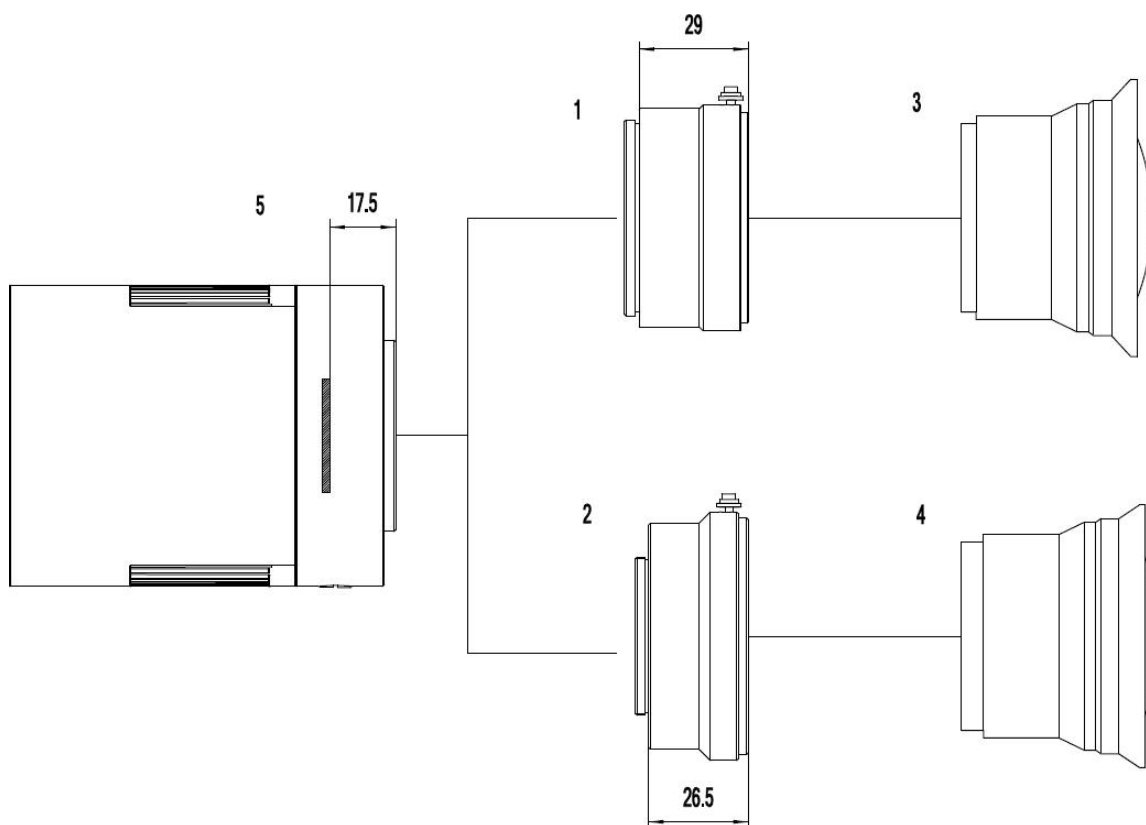
Figure 11 Nikon /Canon Lens with SkyEye Camera
