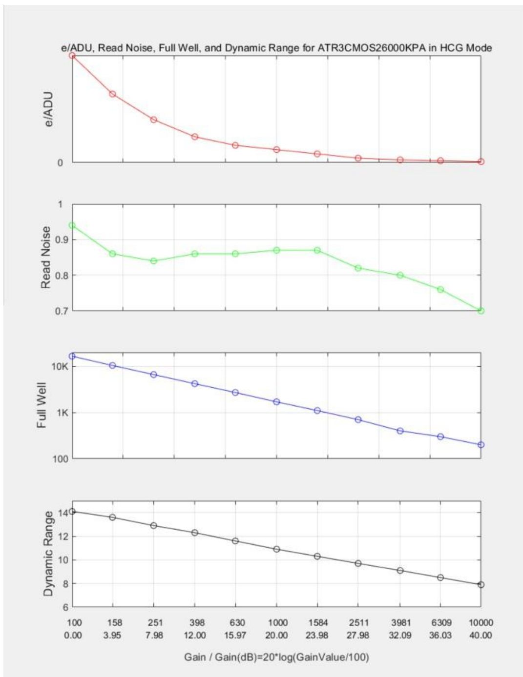
Figure 5 e-/ADU, Read Noise, Full Well and Dynamic Range for SkyEye26AM-plus
