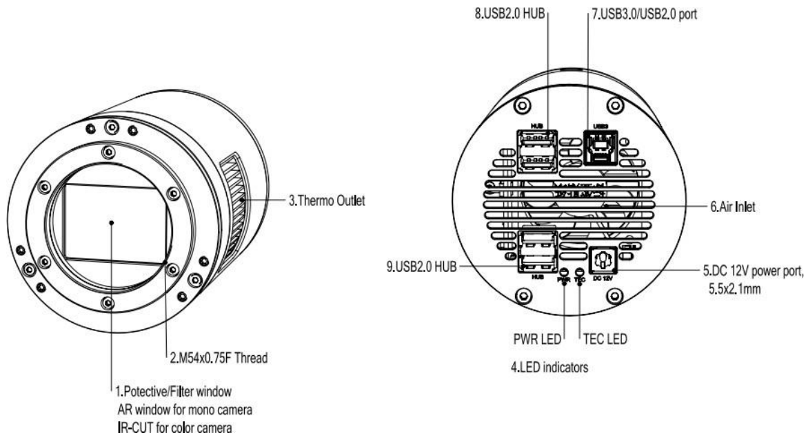
Figure 9 Camera Outline and Interface.
