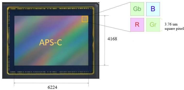
Figure 1 IMX571 Sensor and Its Pixel Structure
