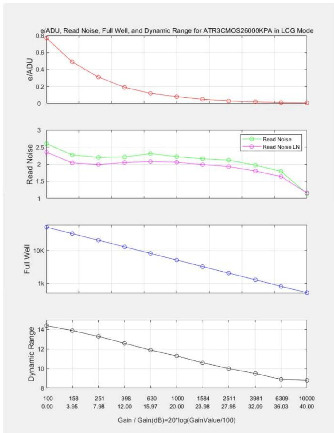
Figure 6 e/ADU, Read Noise, Full Well and Dynamic Range for SkyEye26AM-plus
