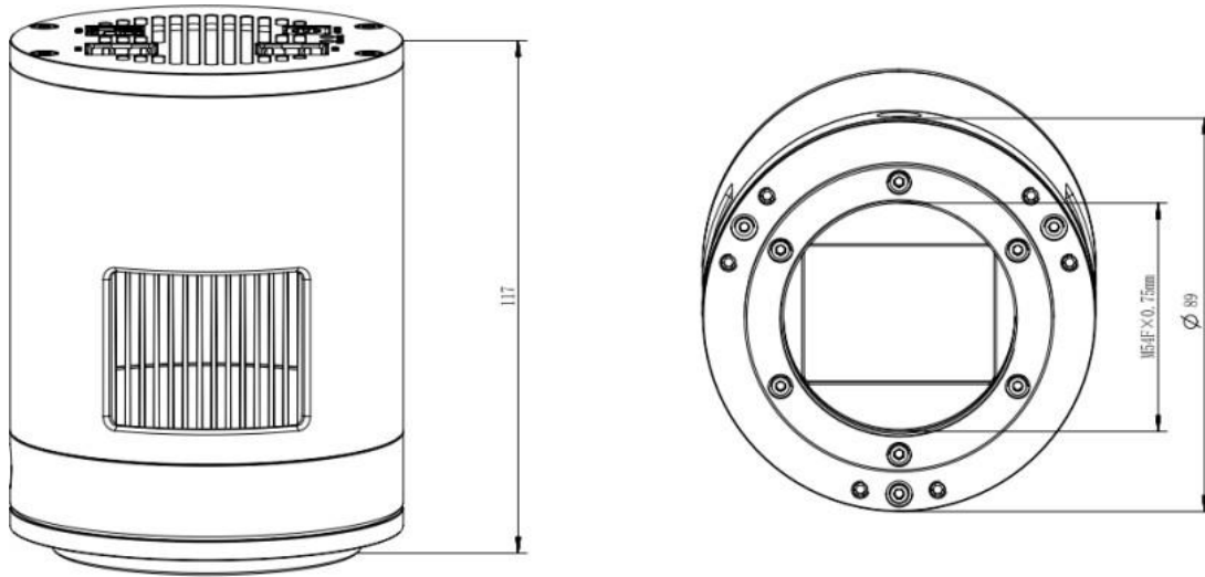
Figure 8 Dimension and Mount of SkyEye26AM-plus
