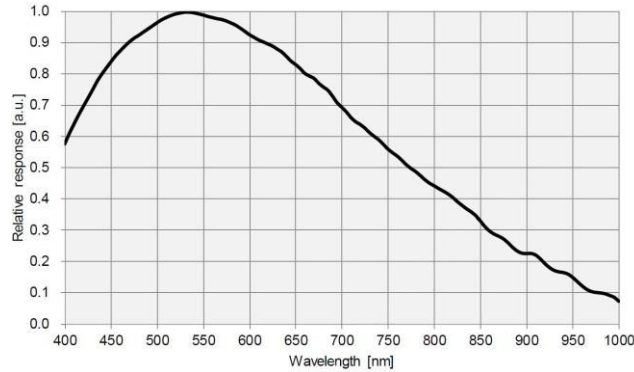
Figure 2 IMX571 Spectral Sensitivity Characteristic
