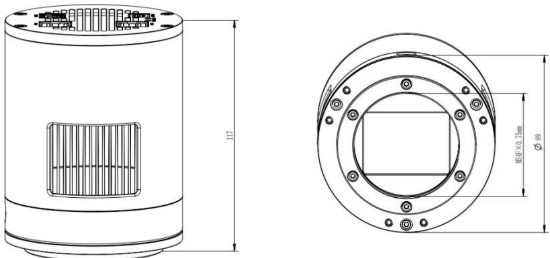
Figure 8 Dimension and Mount of SkyEye26AC-plus
